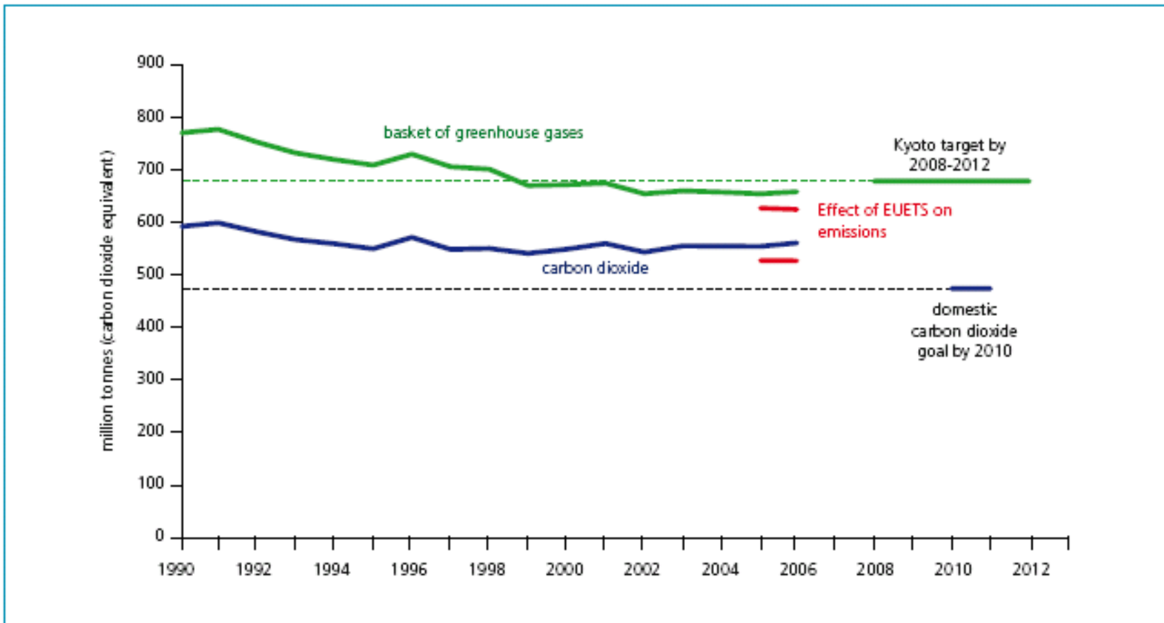
Figure 2: Effects of EU ETS on UK greenhouse gas emissions 1990–2006 (2006 results are provisional)
